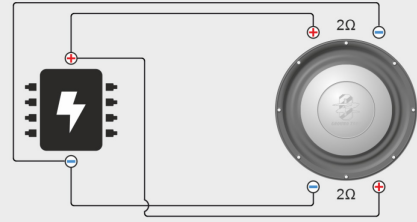
Serial wiring → 4 Ohms
