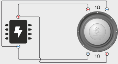
Serial wiring → 2 Ohms
