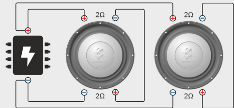
Parallel / serial mixed wiring → 2 Ohms
