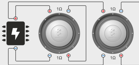
Parallel / serial mixed wiring → 1 Ohm
