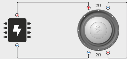
Serial wiring → 4 Ohms
