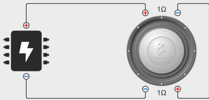
Serial wiring → 2 Ohms
